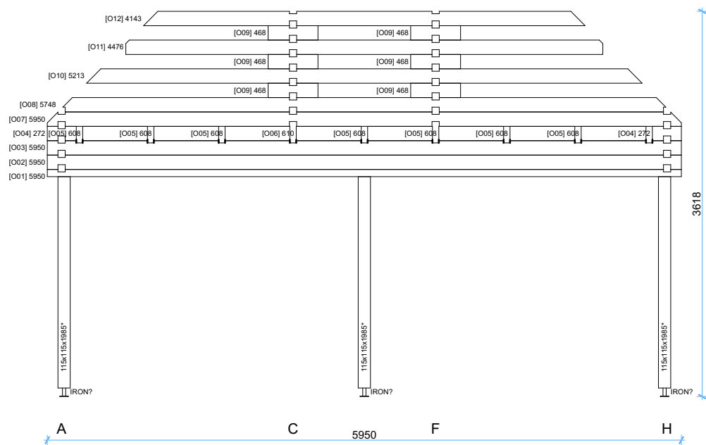
Wall O
