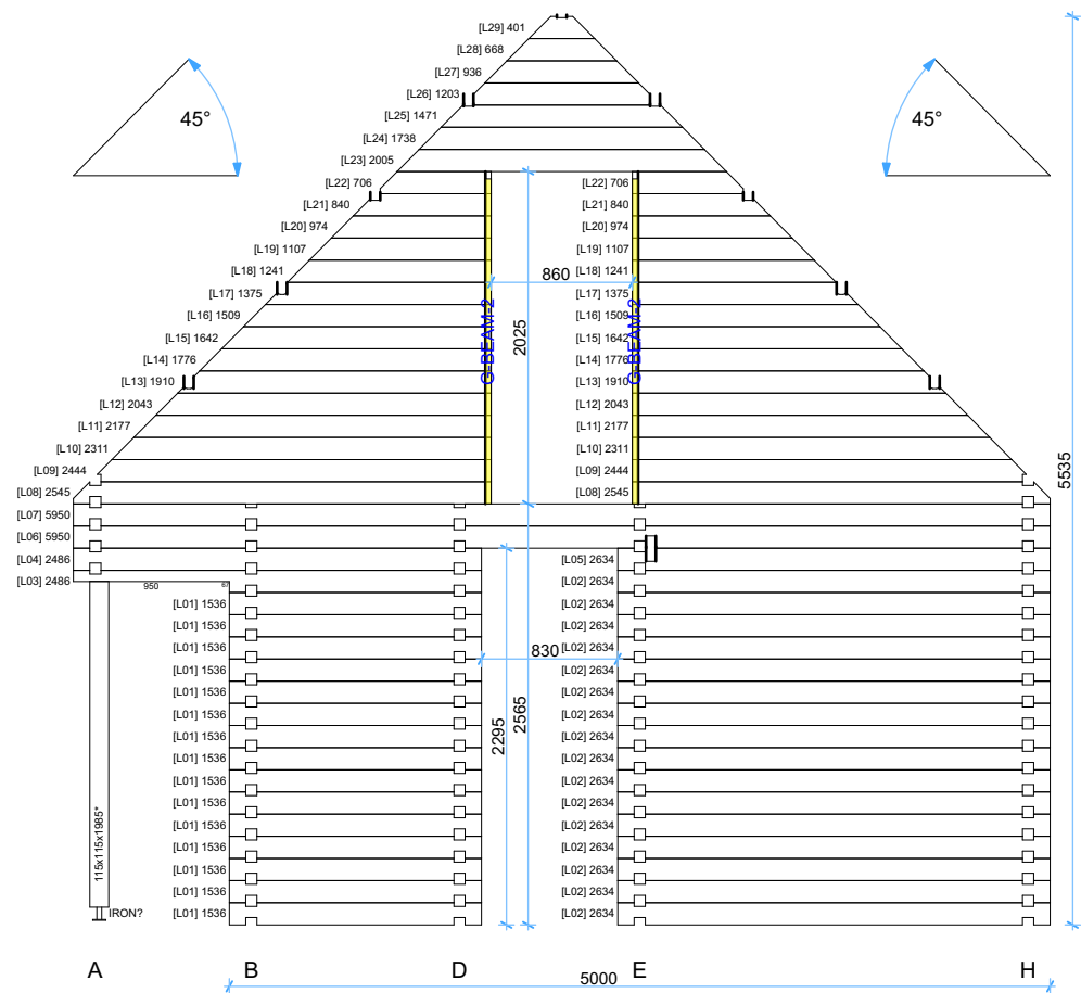
Wall L
