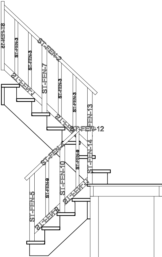
Stairs Fence-1
