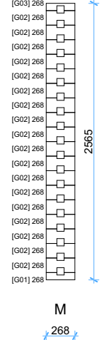
Wall G 1:50
