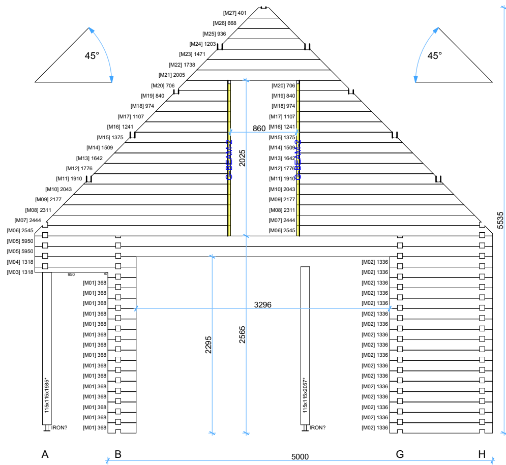
Wall M
