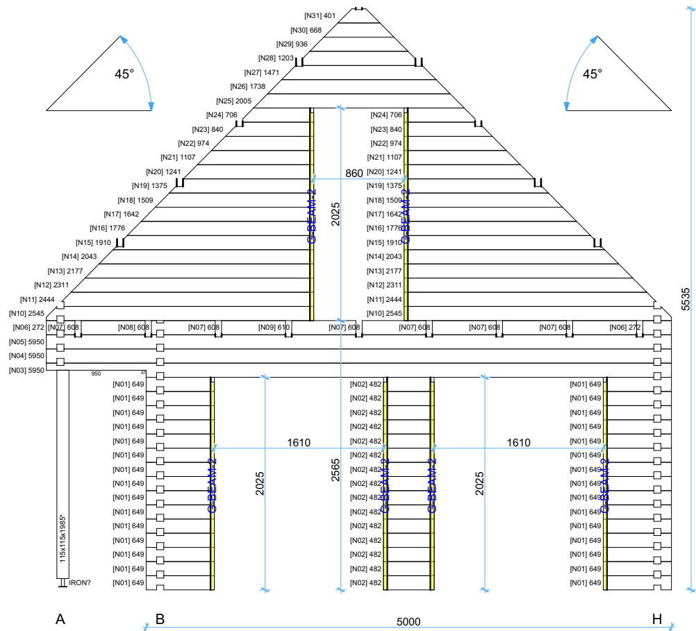
Wall N
